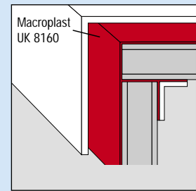
Bonding of panels and sidewall assembly of superstructures
