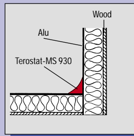
Sealing of sandwich elements in coldstores
