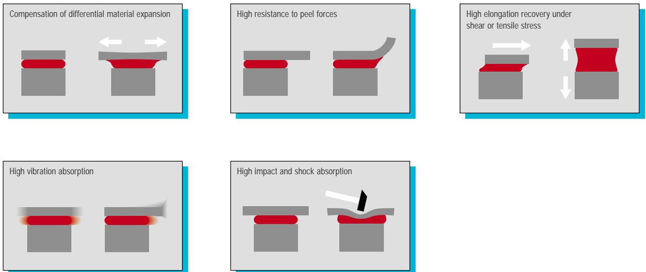
Figure 1: Advantages of elastic bonding and sealing
