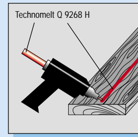
Application by means of a hot melt gun
